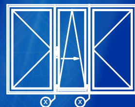
Schematic: G Fixed / Sliding / Fixed Turn* / Sliding / Turn*
