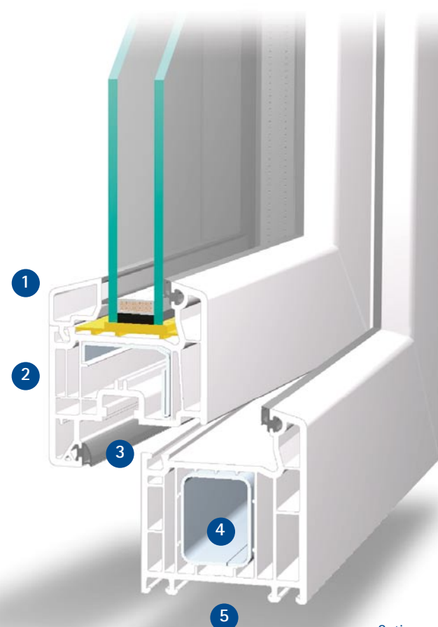
Option: Recessed sash
